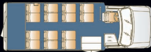
158" W.B. 23' 14 Passenger and Rear Luggage
