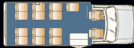
138" W.B. 21' 14 Passenger with Co-Pilot and Cargo Space
