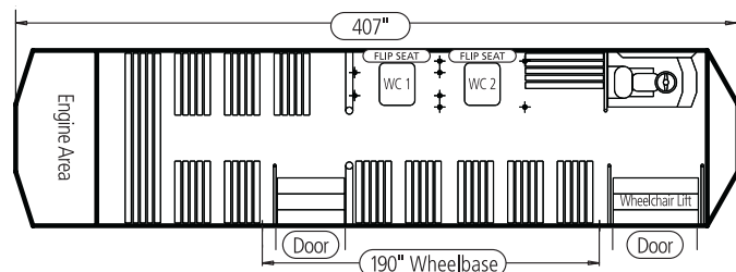
Mainstreet 190 Basic Floorplan
