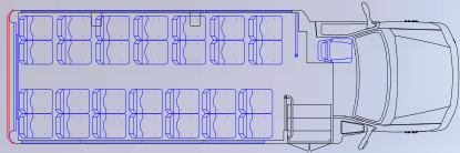
29'; No Lift; 28 Passengers + Driver
