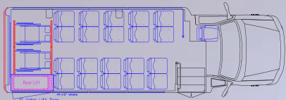
29'; Rear Lift; 20 Passengers + Driver
