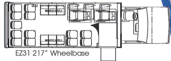
EZ31 217" Wheelbase
